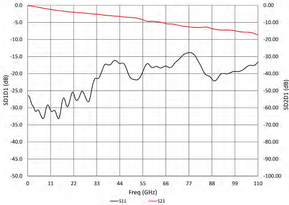
100 Ohm Differential Insertion Loss to 110 GHz (ISB110)
