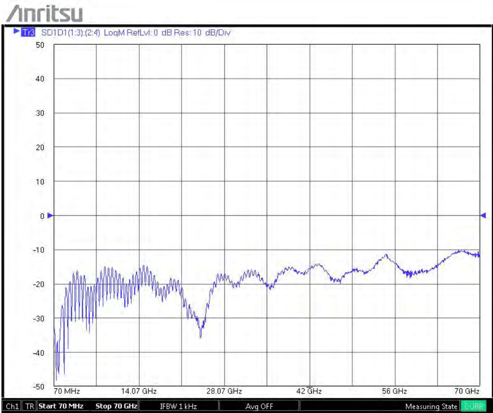
100 Ohm Single-Ended Return Loss to 70 GHz (DB67-002/003)
