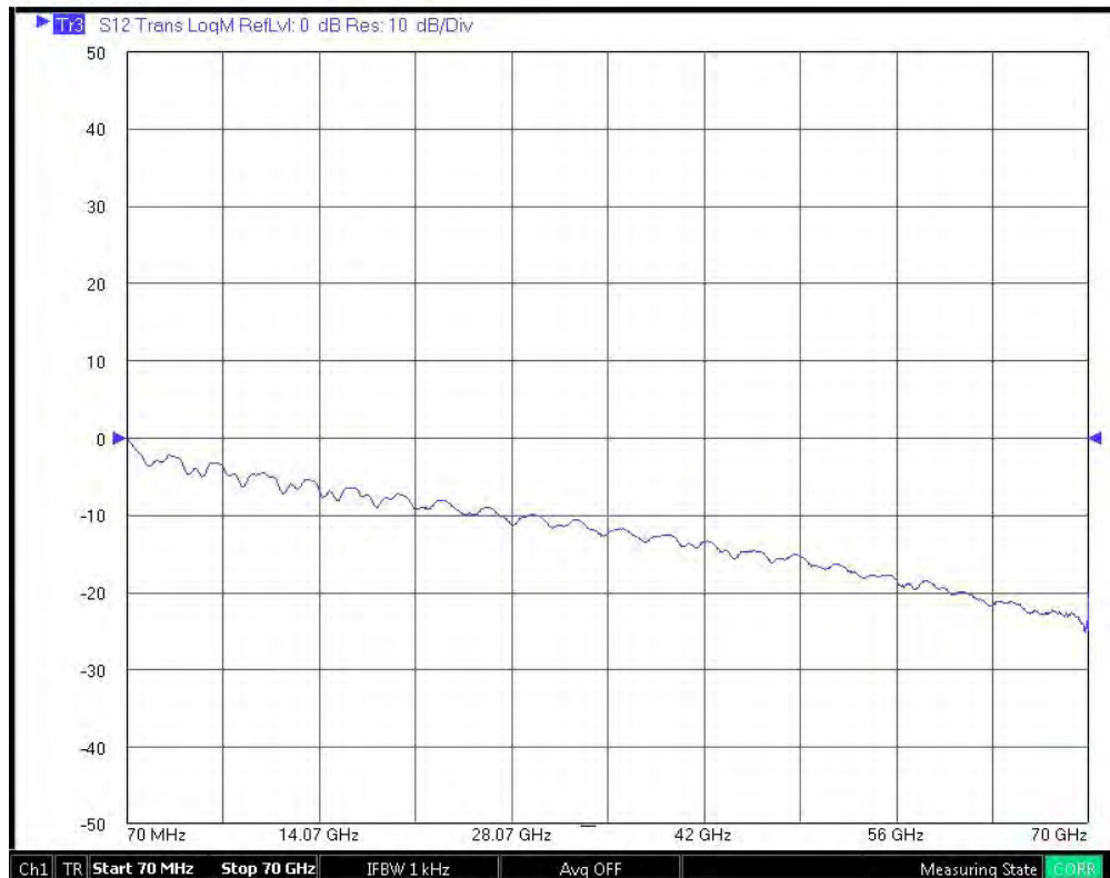
50 Ohm Beatty Line Insertion Loss to 70 GHz (DB67-002/003)
