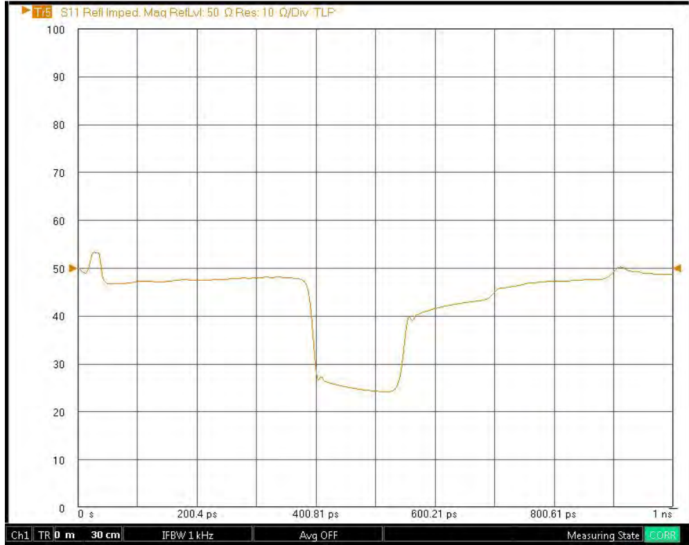
50 Ohm Beatty Line Impedance Plot (DB67-002/003)
