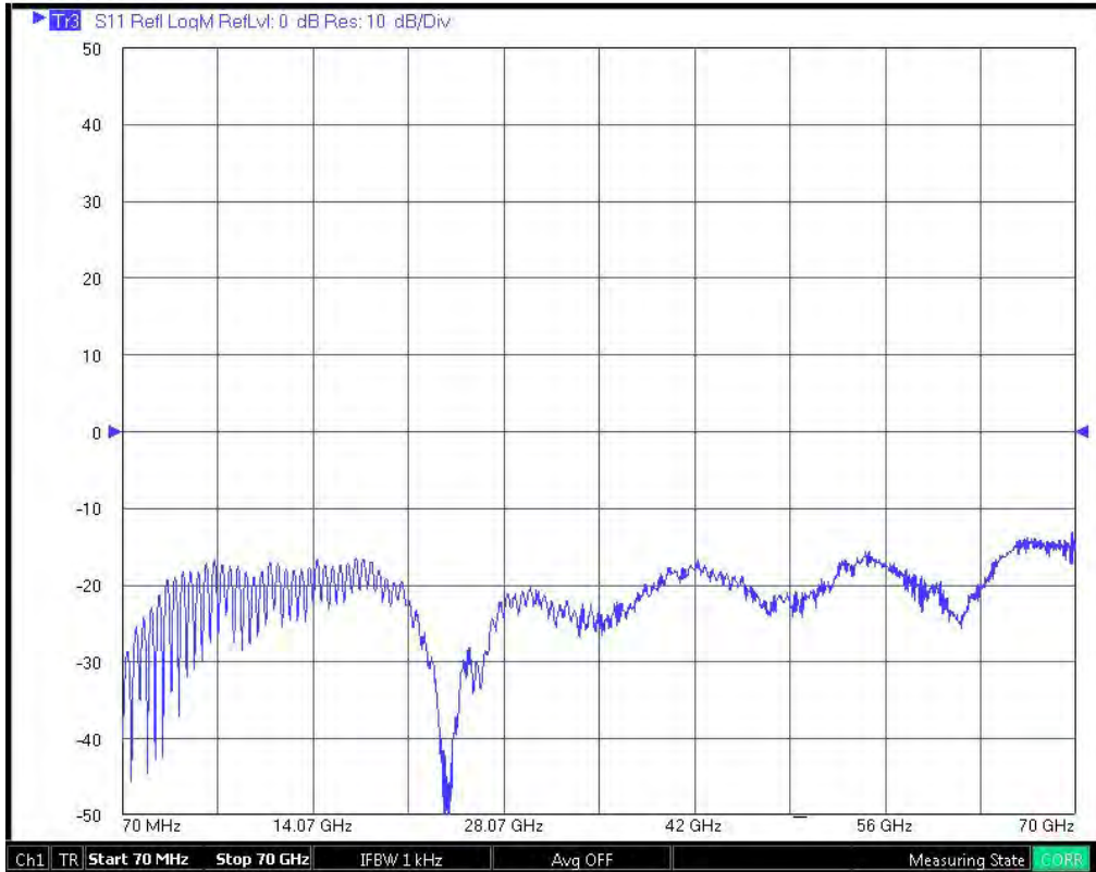
50 Ohm Return Loss to 70 GHz (DB67-002/003)
