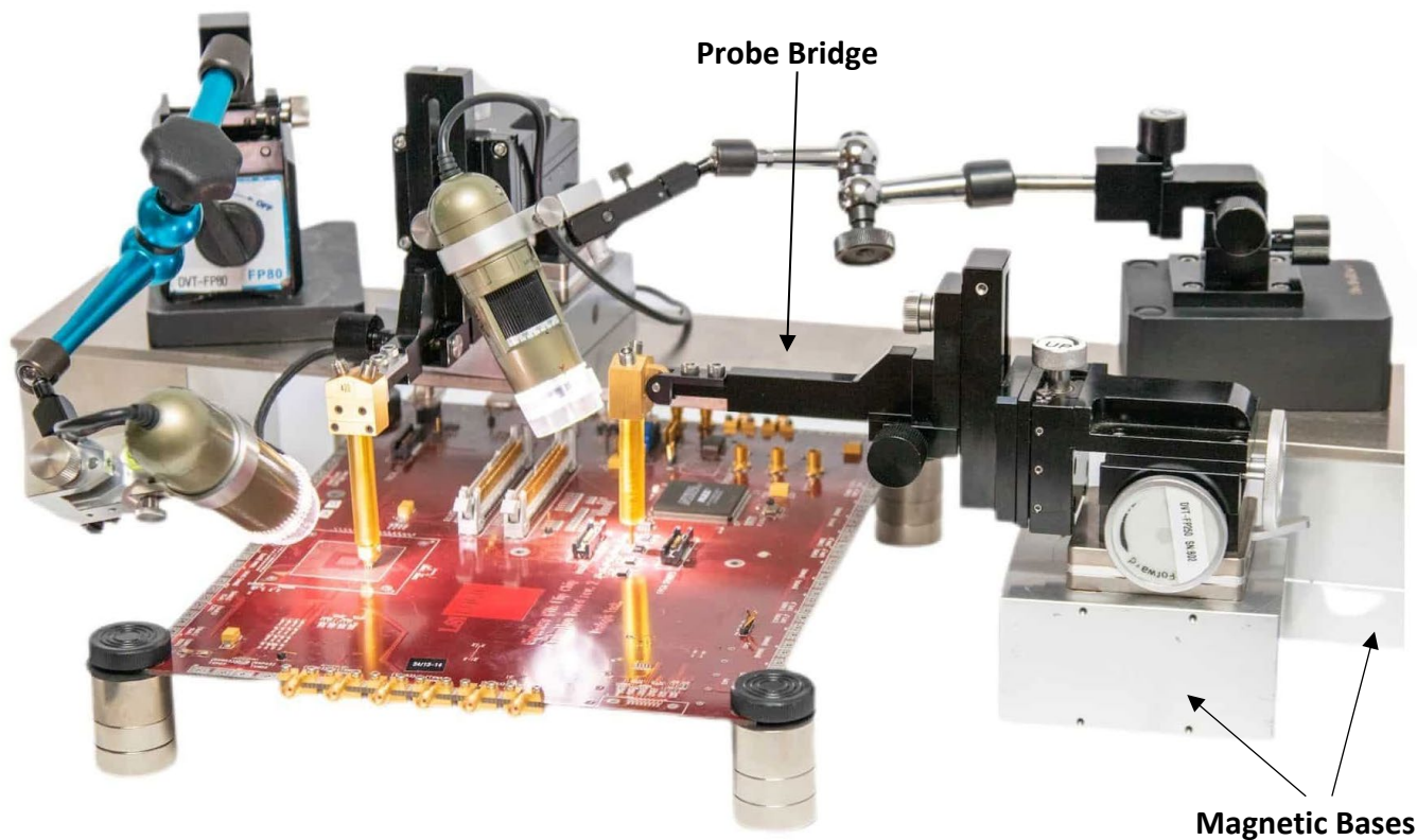
Complete system illustrating use of DVT-FP100 Magnetic Bases.
